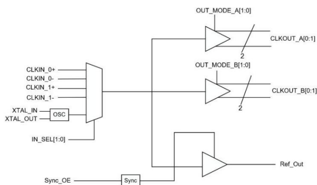
Figure 1 Functional Diagram
